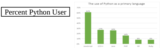
Figure 1 Use of Python as a Primary Language (Python Developers Survey 2016: Findings)
