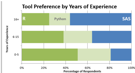
Figure 9 Depicts Tool Preference by the Years of Experience ( http://www.burtchworks.com/2017/06/19/2017-sas-r-python-flash-survey-results/ )
