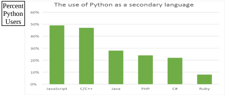
Figure 2 Use of Python as a Secondary Language (Python Developers Survey 2016: Findings)
