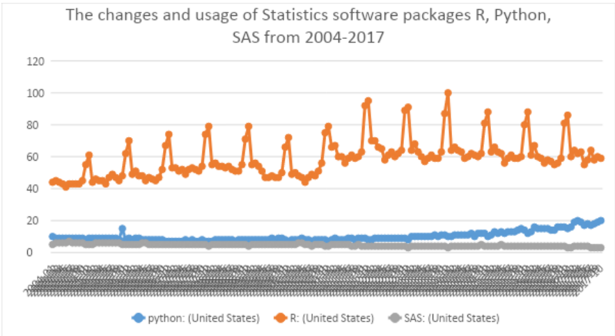
Figure 13 The use of Software Packages and how they have changed over the Years ( https://trends.google.com/trends/explore?date=all&geo=US&q=python, R, SAS )
